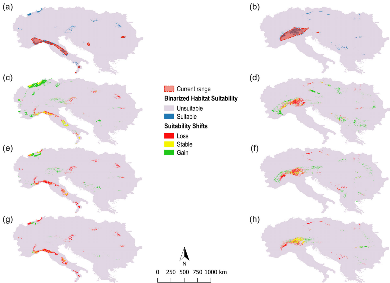
Fig. 4. Suitable areas under the current scenario, obtained from the predictions of the weighted mean EM, and \alpha -hull-based current range (hatched polygons) for (a) N. corpulenta and (b) N. rhaetica ; predicted shifts in HS by 2070 under RCPs 2.6, 4.5 and 8.5 for (c), (e) and (g) N. corpulenta , and (d), (f) and (h) N. rhaetica , respectively. [Color figure can be viewed at wileyonlinelibrary.com ]
