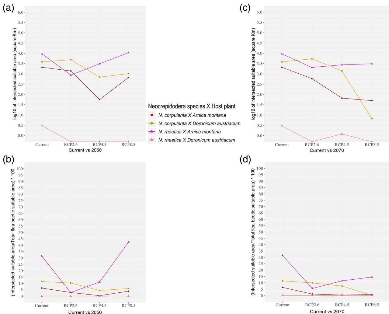
Fig. 7. Variation in the extent of overlapping suitable area between N. corpulenta , N. rhaetica and the corresponding candidate host plants ( Arnica montana and Doronicum austriacum ) from the current scenario to 2050 (a) and 2070 (c) under the three RCPs; variation in the percent extent of overlapping suitable area with respect to the overall suitable area for the flea beetle under the different RCPs in 2050 (b) and 2070 (d). [Color figure can be viewed at wileyonlinelibrary.com ]
