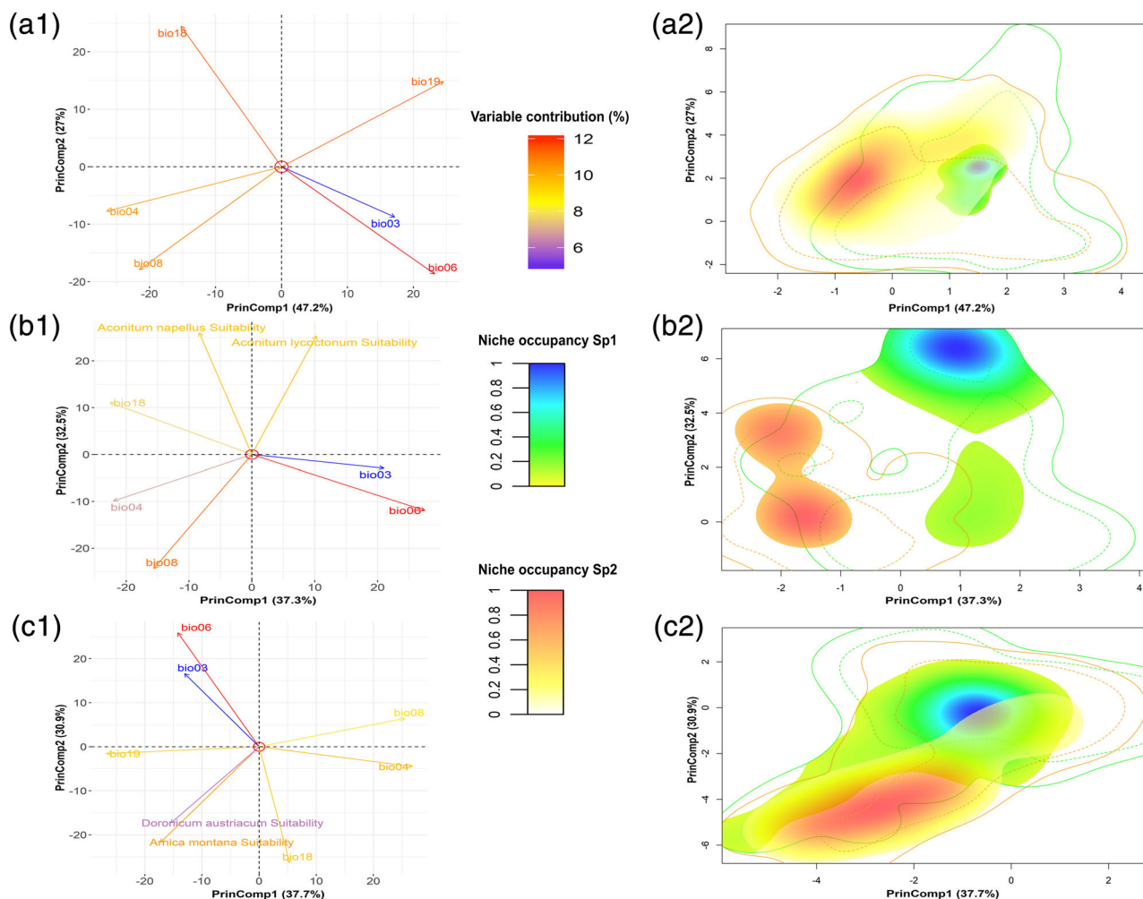
Fig. 5. Contributions of the input predictors along the first two principal components ('PCA-env', Broennimann et al. , 2012) for: (a1) N. ligurica and N. melanostoma ; (b1) N. cyaneus concolor and N. cyaneus cyaneus ; (c1) N. corpulenta and N. rhaetica . Density of occurrence in the environmental space defined by the principal components for: (a2) N. ligurica (Sp1) and N. melanostoma (Sp2); (b2) N. cyaneus concolor (Sp1) and N. cyaneus cyaneus (Sp2); (c2) N. corpulenta (Sp1) and N. rhaetica (Sp2). Within the density plots, solid contour lines represent the full environmental background and dashed contour lines represent 50% of the background environment. [Color figure can be viewed at wileyonlinelibrary.com ]
