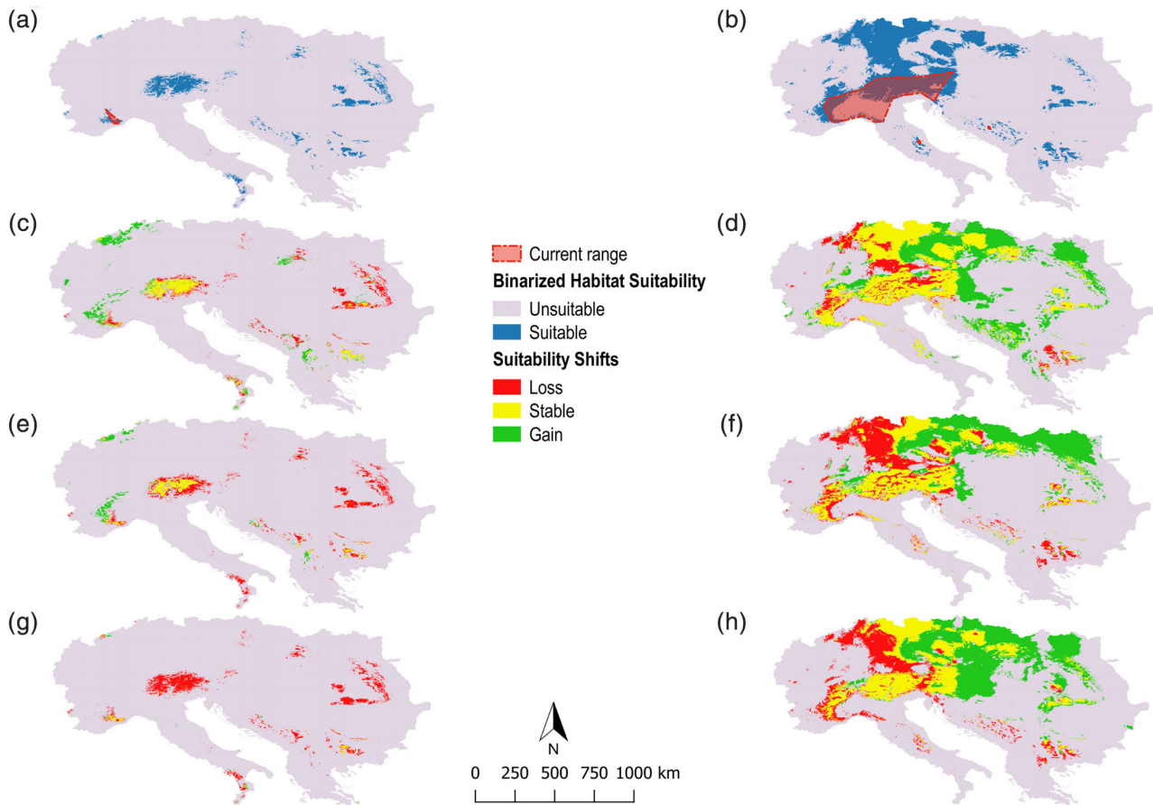
Fig. 2. Suitable areas under the current scenario, obtained from the predictions of the weighted mean EM, and \alpha -hull-based current range (hatched polygons) for (a) N. ligurica and (b) N. melanostoma ; predicted shifts in HS by 2070 under RCPs 2.6, 4.5 and 8.5 for (c), (e), and (g) N. ligurica , and (d), (f) and (h) N. melanostoma , respectively. [Color figure can be viewed at wileyonlinelibrary.com ]
