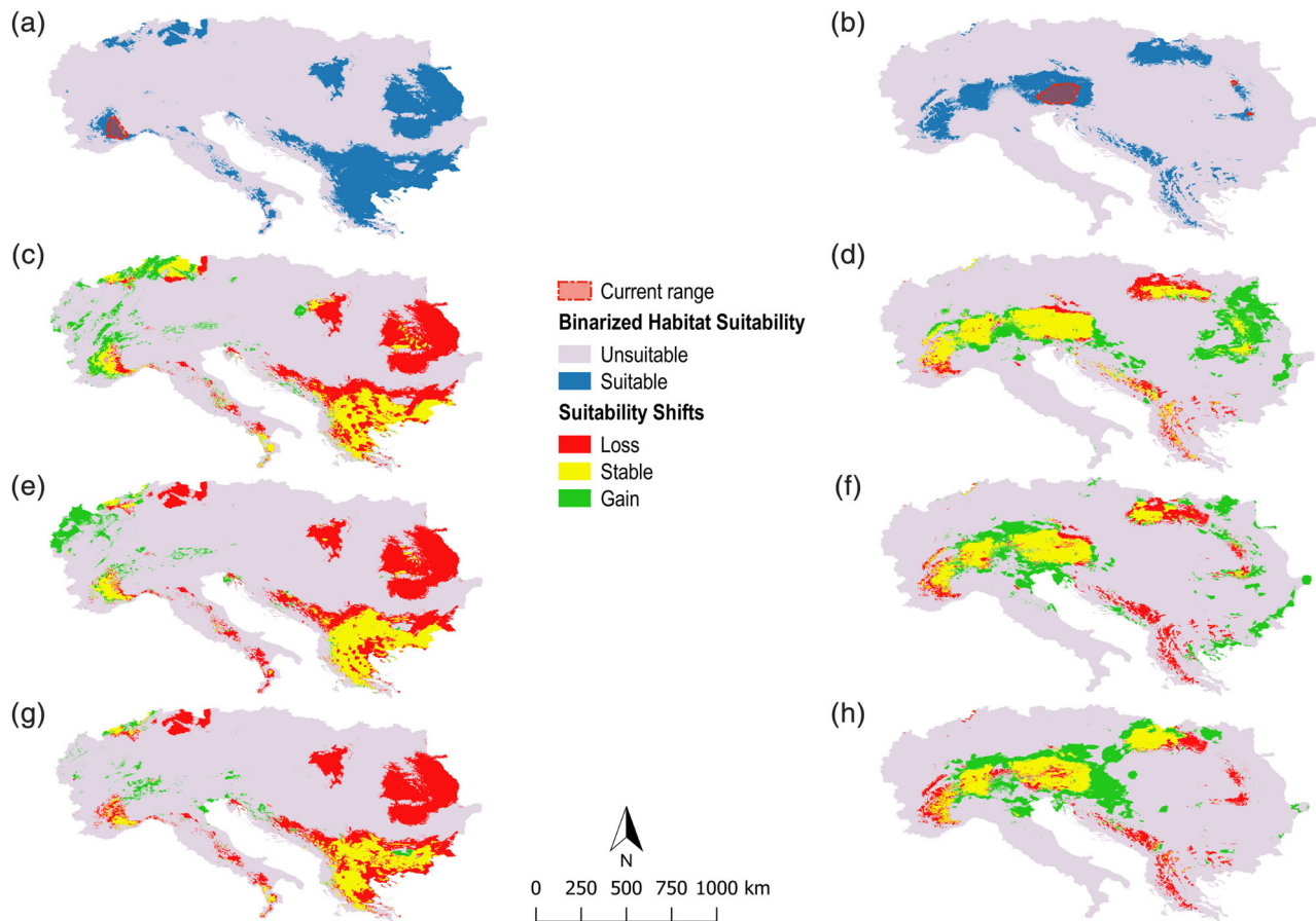
Fig. 3. Suitable areas under the current scenario, obtained from the predictions of the weighted mean EM, and \alpha -hull-based current range (hatched polygons) for (a) N. cyanescens concolor and (b) N. cyanescens cyanescens ; predicted shifts in HS by 2070 under RCPs 2.6, 4.5 and 8.5 for (c), (e) and (g) N. cyanescens concolor , and (d), (f) and (h) N. cyanescens cyanescens , respectively. [Color figure can be viewed at wileyonlinelibrary.com ]
