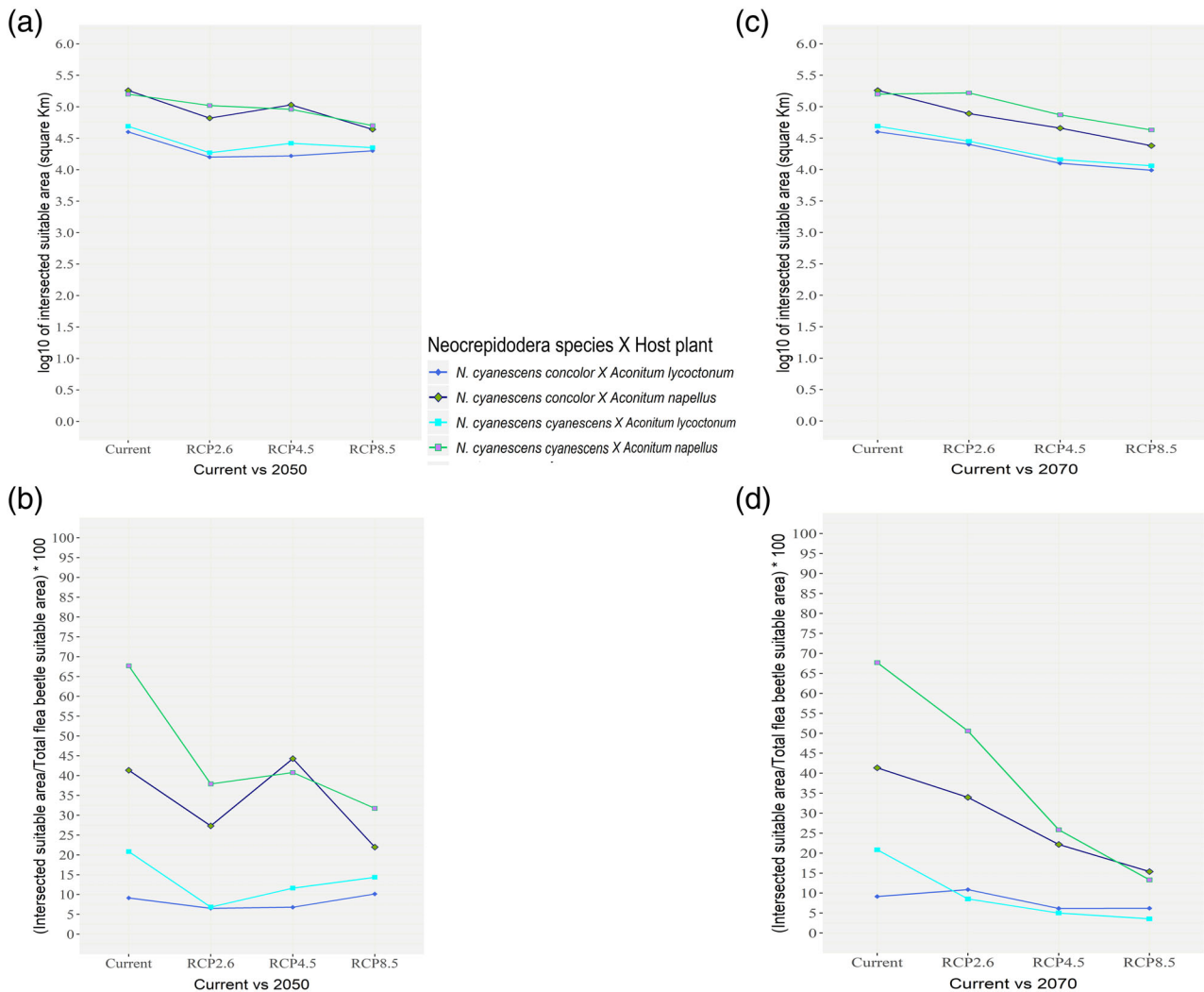
Fig. 6. Variation in the extent of overlapping suitable area between the two N. cyanescens subspecies and the corresponding candidate host plants ( Aconitum lycoctonum and A. napellus ) from the current scenario to 2050 (a) and 2070 (c) under the three RCPs; variation in the percent extent of overlapping suitable area with respect to the overall suitable area for the flea beetle under the different RCPs in 2050 (b) and 2070 (d). [Color figure can be viewed at wileyonlinelibrary.com ]
