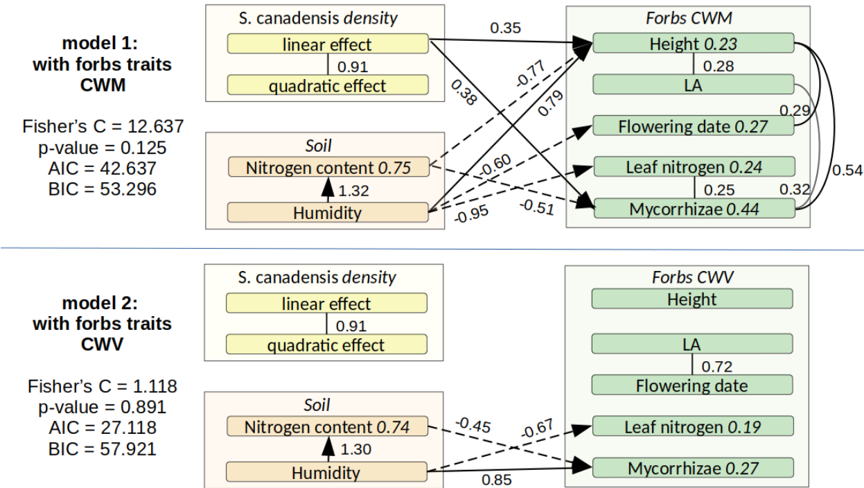
Figure 3: Structural equation models representing the impact of S. canadensis density on trait means (CWM, model 1) and variances (CWV, model 2) of forb species. Black solid and dashed arrows represent significant positive and negative directed impacts ( p -value < 0.05 ), respectively. Black lines represent significant positive undirected relationships ( p -value < 0.05 ). The coefficients associated with each significant link are indicated beside the corresponding arrows and lines, and the values beside the response variables are their associated marginal R^2 . The structure of the initial model (i.e., before variable and link selection) is shown on Figure 2. Some links were removed (when not significant) and others added (to support independence claims) to the initial models following the model building procedure described in Materials and Methods.
