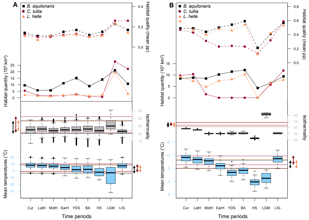
Figure 6. Changes in climate suitability over time in (A) Europe and (B) the Jura massif.
