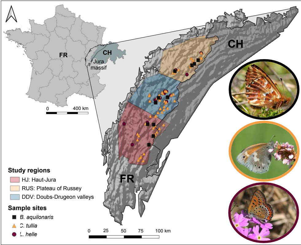
Figure 1. Study area and location of sample sites for the three species. The top left map shows the context of the study area, locating the Jura massif on the border between France (FR) and Switzerland (CH). The enlarged map shows the Jura massif with the three main study regions (HJ; RUS; DDV) in different transparent fill colors. Symbol shape and colors represent the location of sample sites for each species. Photos credits: B. aquilonaris , Frédéric Mora; C. tullia , Mathilde Poussin; L. helle , Pierre Durllet.
