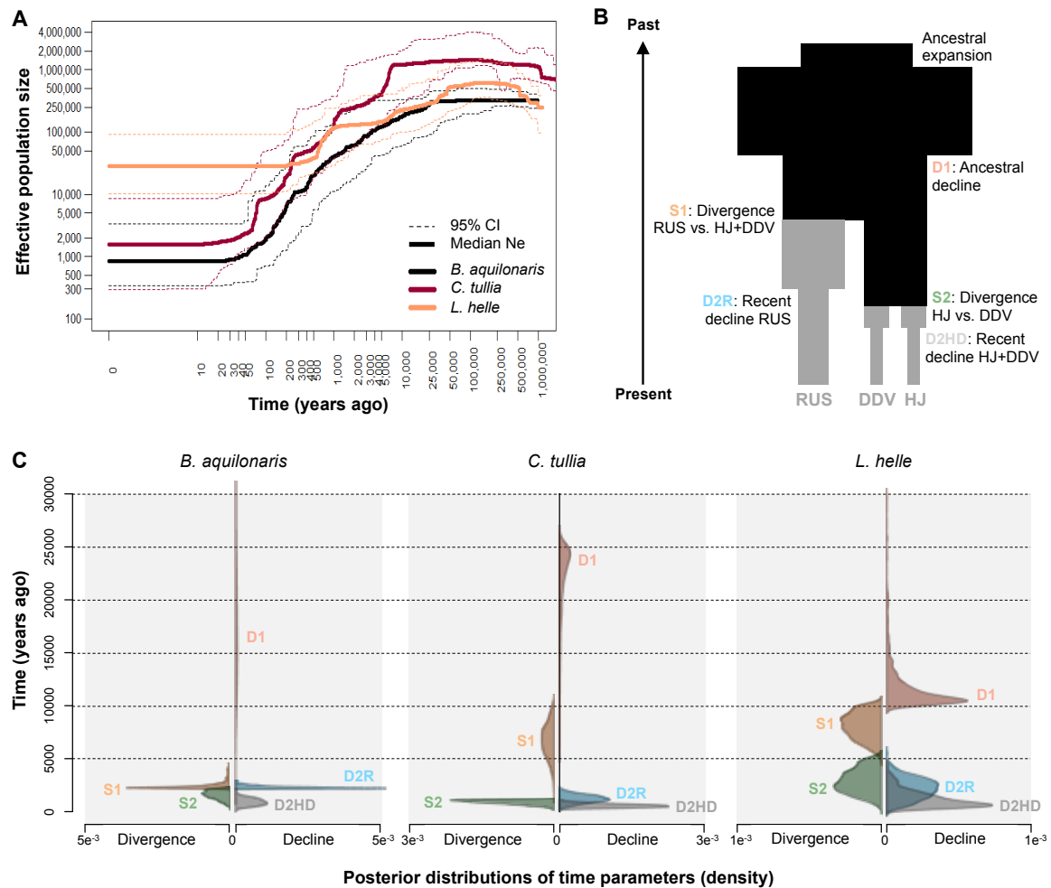
Figure 4. Population demographic history. A) Changes in effective population size ( N_e ) over time based on the species-level SFS (all regions combined) using Stairway Plot v2. Full-colored lines: median N_e ; dotted lines: 95% confidence intervals (CI) generated from 200 bootstrap replicates (population-level analyses in Supplementary Figure S5). B) Schematic representation of the best divergence scenario for the three species using DIYABC (see Table 2 for identification of best scenario). C) Estimated divergence and decline times for the best scenario presented in B (posterior distributions for the 1% simulated data closest to the observed data).
