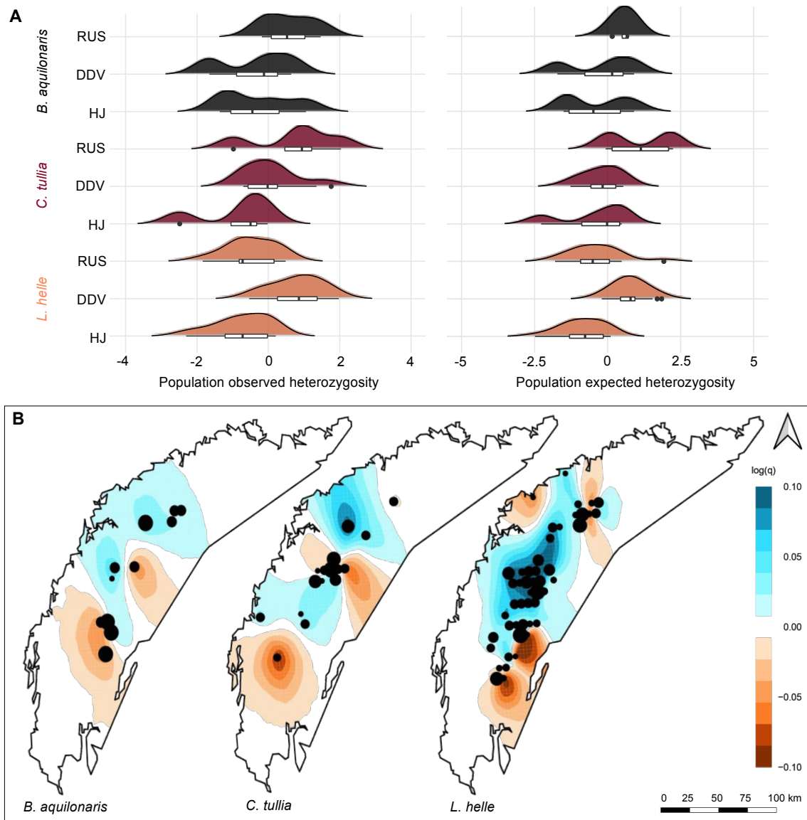
Figure 2. Spatial patterns in genetic diversity. A) Density and distribution of observed ( H_o ) and expected ( H_e ) heterozygosity (scaled and centered separately for each species) among the three regions, from North (RUS) to South (HJ). B) EEMS contour plots of the average posterior distribution of diversity rates q ( \log_{10} scale). Darker font colors show significantly high (blue) or low (brown) within-deme genetic dissimilarities.
