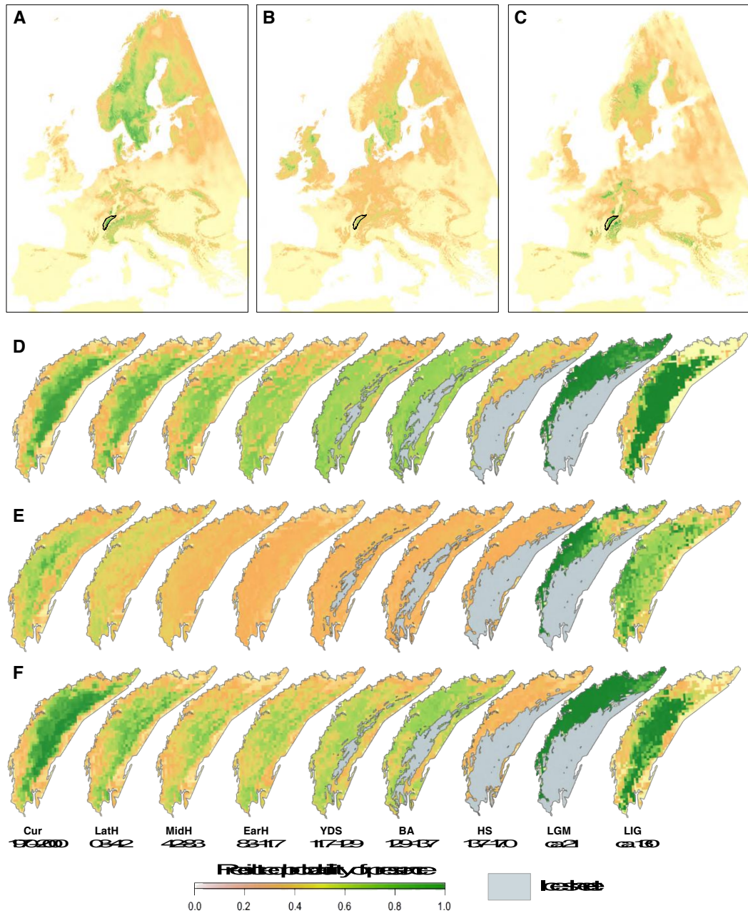
Figure 5. Changes in species potential distribution over time in the Jura massif. Species potential distribution at the European scale based on six bioclim variables (BIO1, BIO2, BIO3, BIO8, BIO12, BIO15) under current conditions for A) B. aquilonaris B) C. tullia and C) L. helle . Predicted distributions under current climate (Cur) and palaeoclimates in the Jura massif (predicted distributions at the European scale are in Supplementary Figures S6 to S8) for D) B. aquilonaris E) C. tullia and F) L. helle . Paleoclimates (in kya): Late Holocene (LatH); Mid Holocene (MidH); Early Holocene (EarH); Younger Dryas Stadial (YDS); Bølling-Allerød (BA); Heinrich Stadial 1 (HS); Last Glacial Maximum (LGM); Last Interglacial (LIG).
