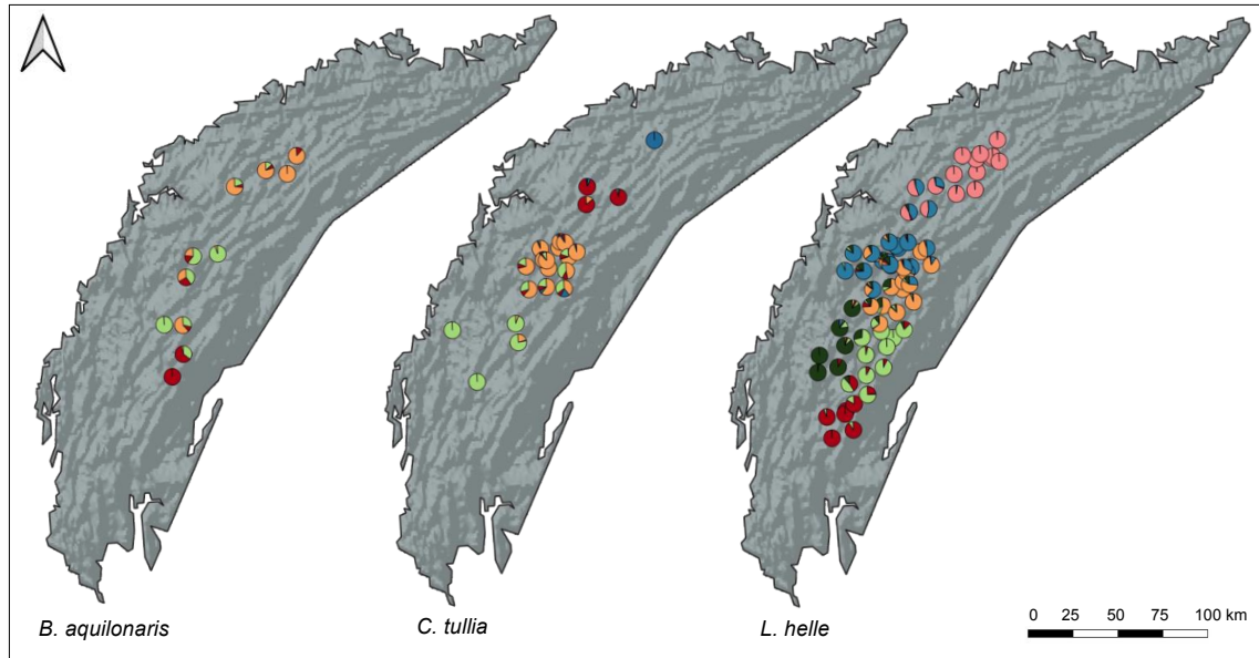
Figure 3. Genetic differentiation among regions. Average ancestry coefficients among individuals per sampling locality, estimated from ADMIXTURE analyses for A) B. aquilonaris (K = 3) B) C. tullia (K=4) and C) L. helle (K=6).
